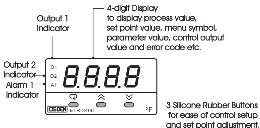
Figure 1.4 Front Panel Layout
